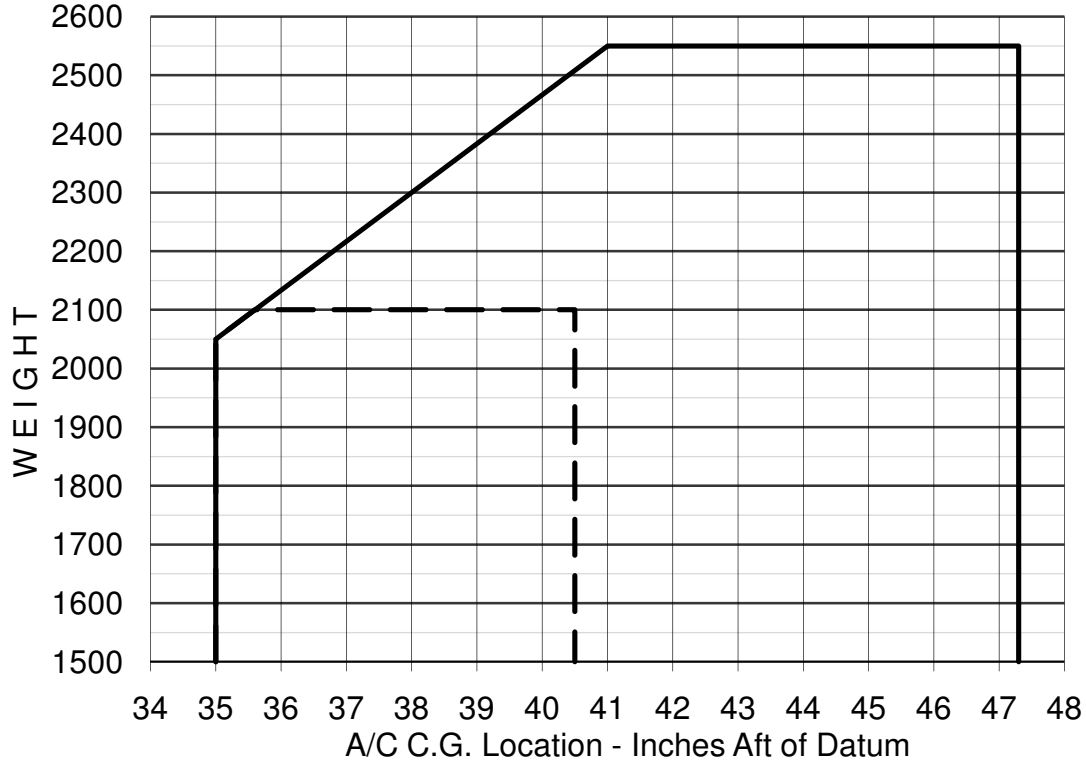
Weight & Balance Chart
